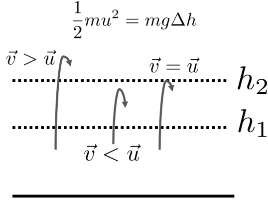
Figure 3: The particles crossing plane h_2 upwards must have had a vertical velocity of at least u (where mg\Delta h = 1/2mu^2 ) as they crossed plane h_1
